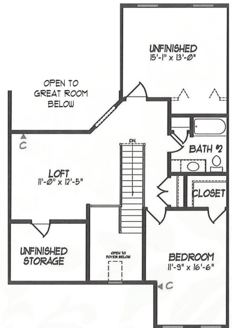
SECOND FLOOR PLAN 661 SF living space
