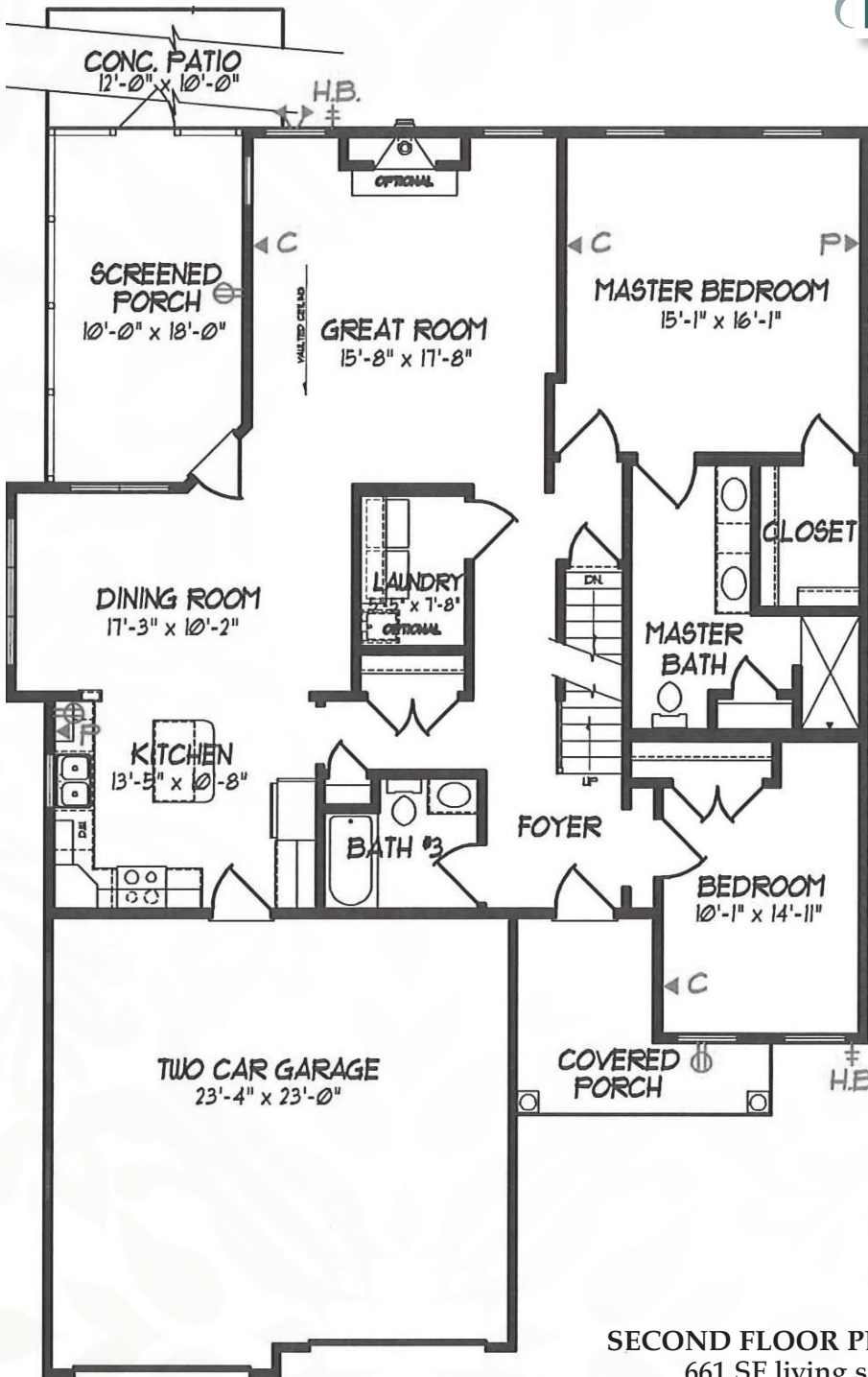
FIRST FLOOR PLAN 1,596 SF living space plus 544 SF garage
